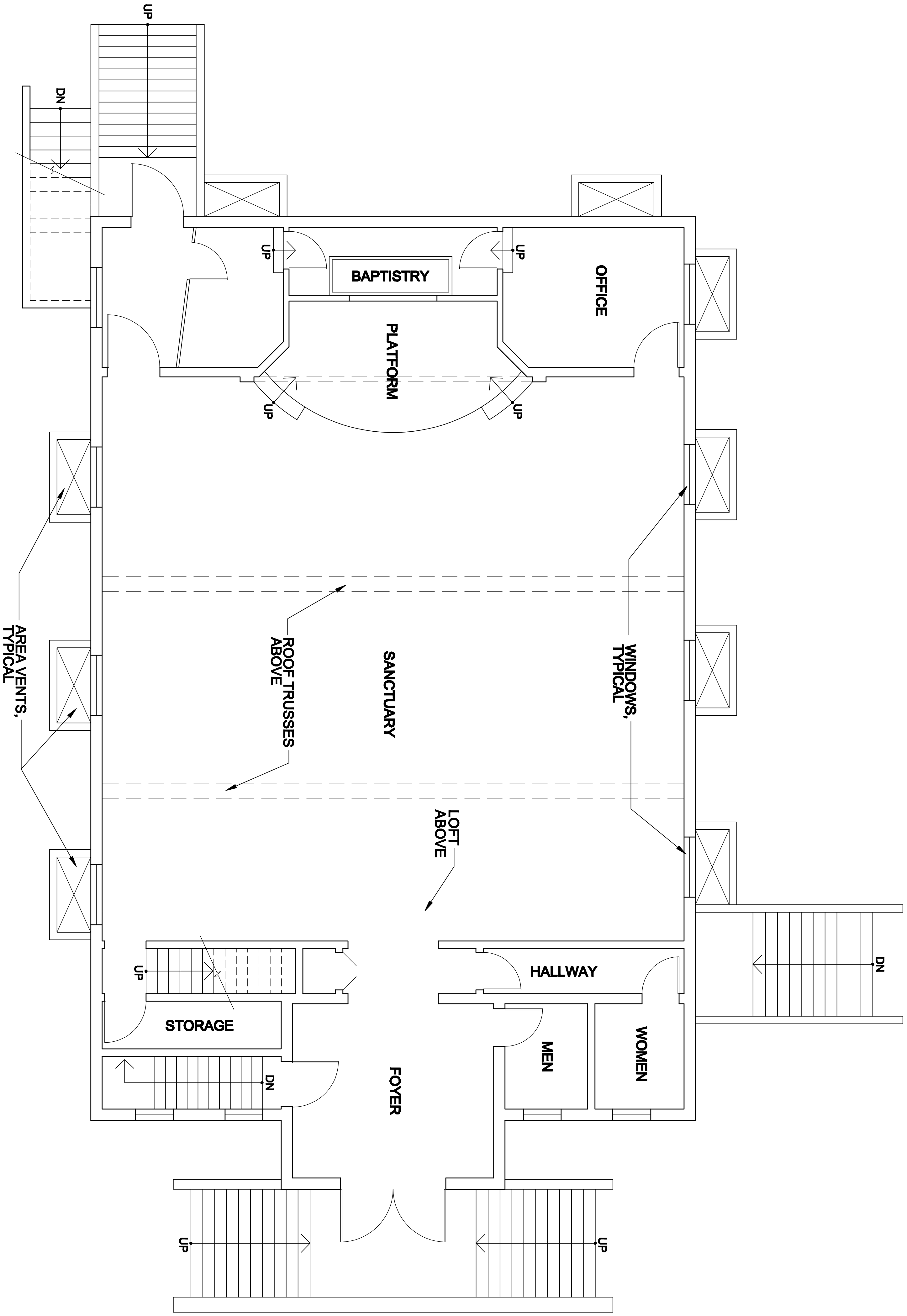
UPPER LEVEL FLOOR PLAN SCALE: 1/4" = 1'-0"
