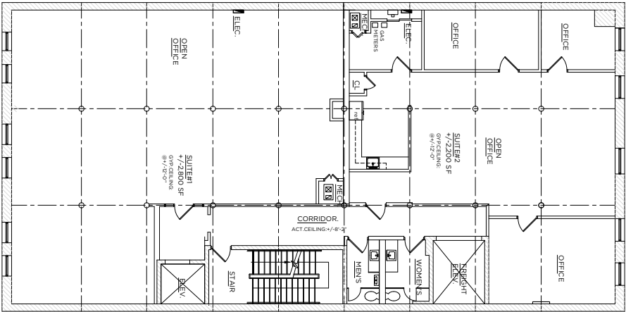
4A FLOOR PLAN
